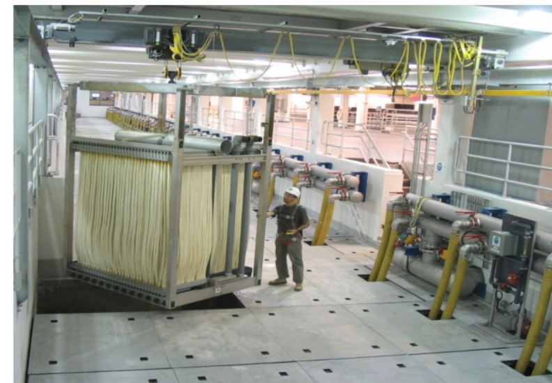
MBR- Submerged type
